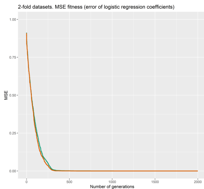
Figure 2: the MSE fitness (mean squared error of the logistic regression coefficients) for the EA for each of the two runs in the twofold split.
